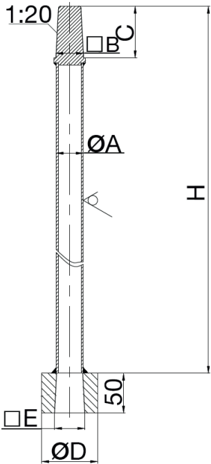
Extension Spindle Dimensions
