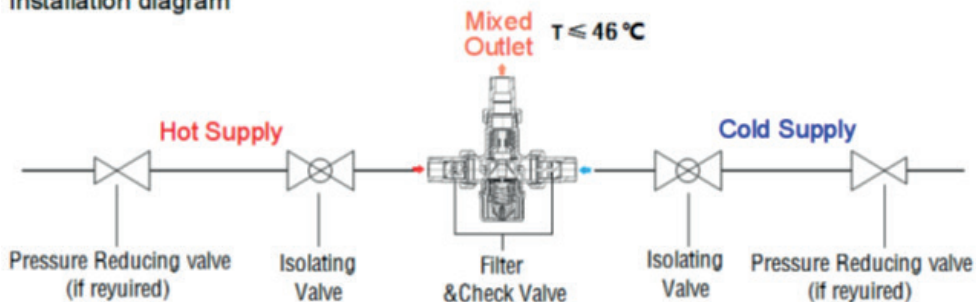
Installation diagram
